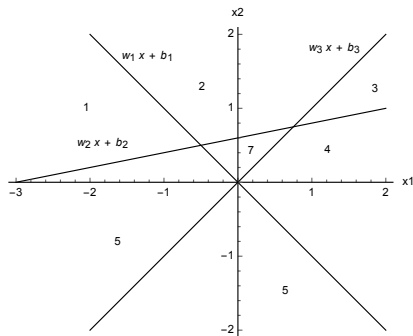
Figure: Hyperplanes defined by three neurons with ReLU activation functions.
