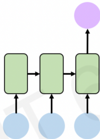
Many to One Sentiment Classification
