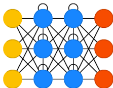
Recurrent
